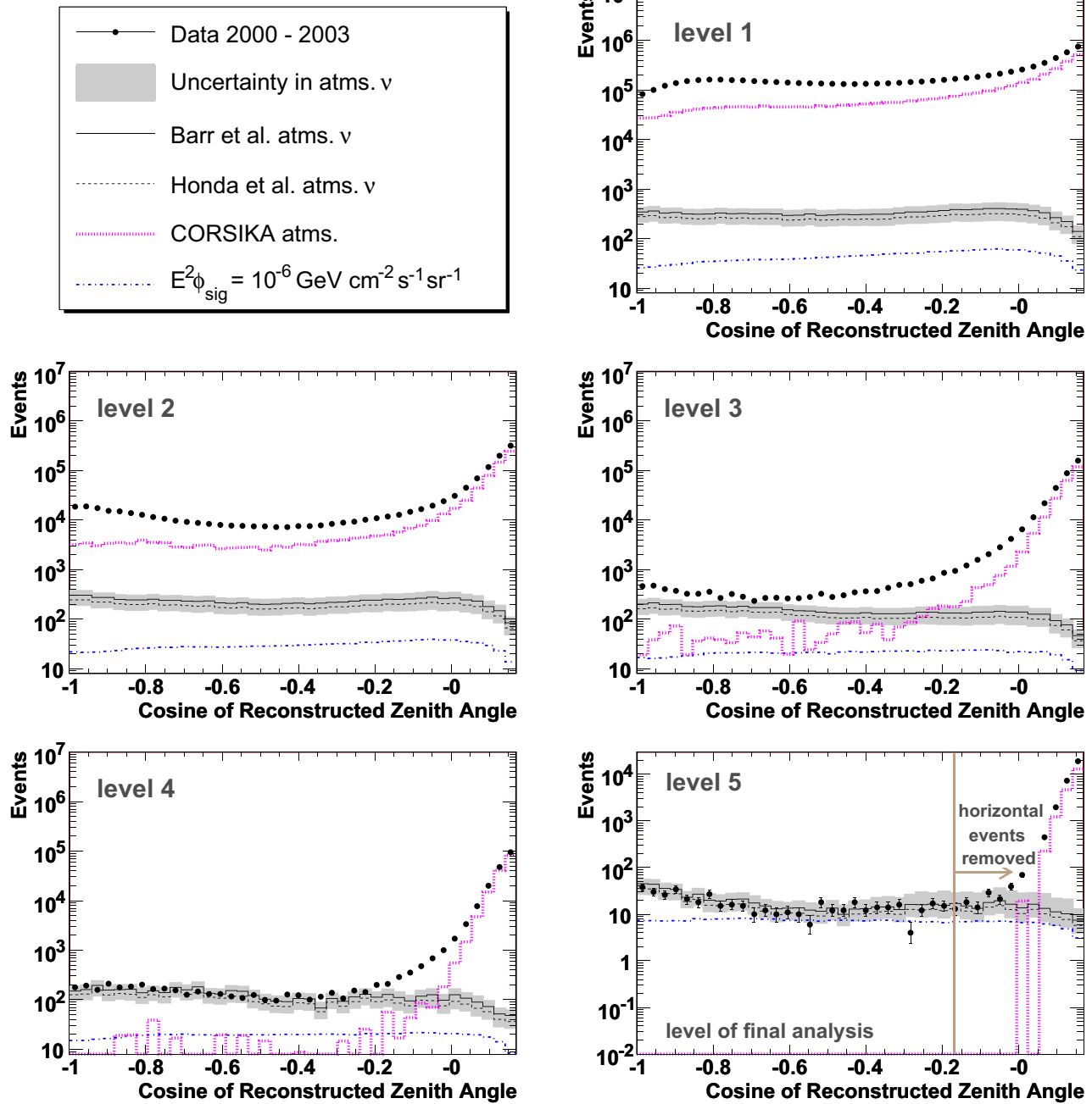
FIG. 3 (color online). The cosine of the zenith angle is plotted for all events surviving the event quality criteria at a given level. Events at \cos(\text{zenith}) = -1 are traveling straight up through the detector from the Northern Hemisphere. The initial zenith angle requirement removed events from 0^\circ to 80^\circ (level 1—top right). Events reconstructed just above the horizon appear at the right side of each plot. Each level represents an increasingly tighter set of quality requirements. As the quality level increased, misreconstructed downgoing muons were eliminated. To ensure a clean upgoing sample, events coming from the horizon were discarded by requiring reconstruction angles greater than 100^\circ . The final analysis was performed at level 5 (bottom right) with horizontal events removed.
